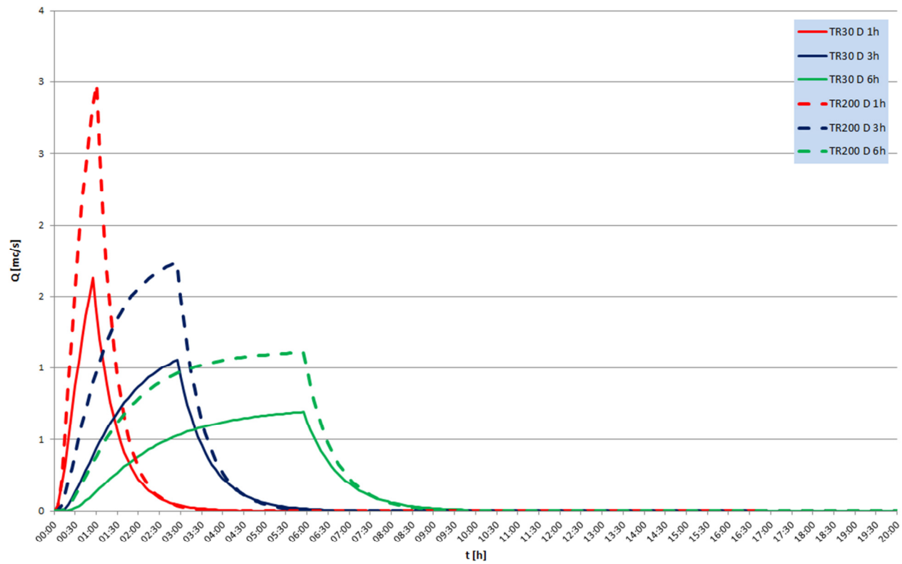
SEZ. 115 - FLOW HYDROGRAPH
