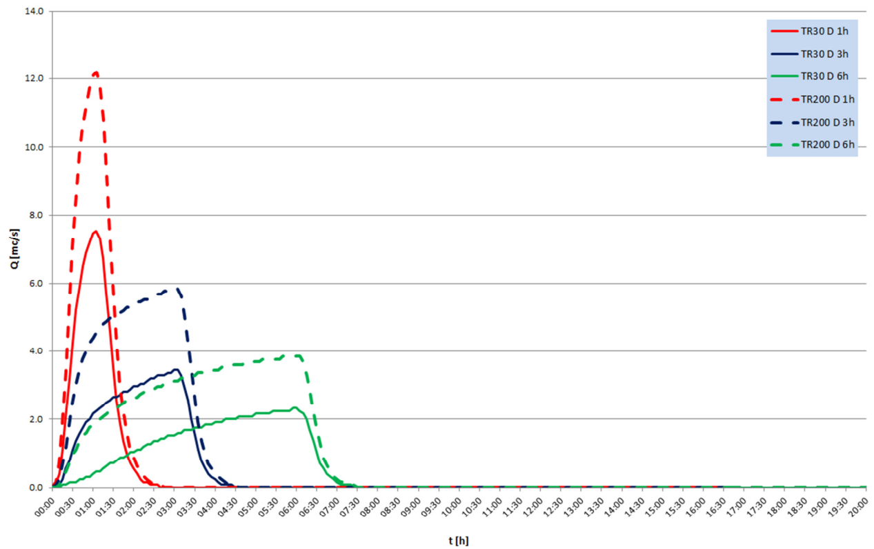
SEZ. 35 - FLOW HYDROGRAPH
