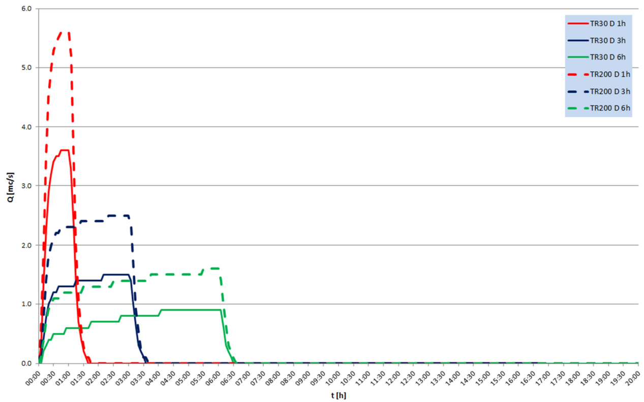
SEZ. 2388 - LATERAL INFLOW HYDROGRAPH
