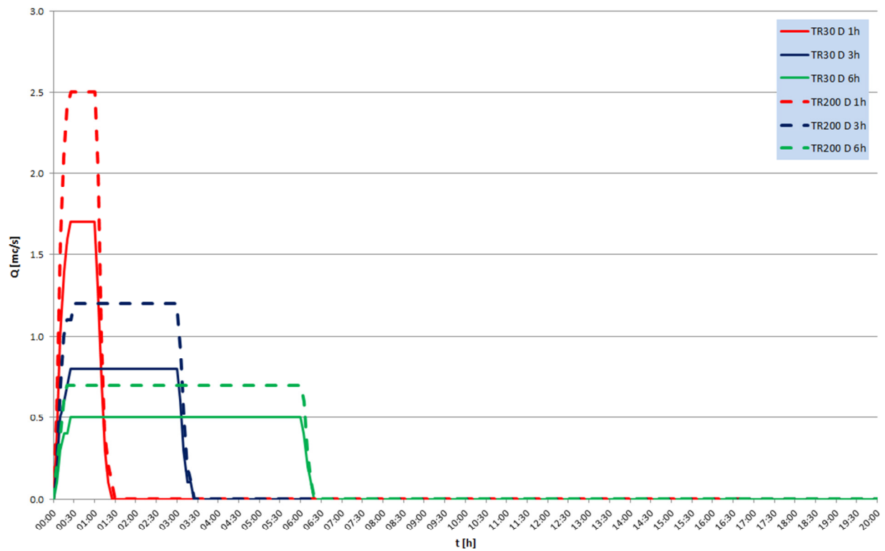
SEZ. 2800 - LATERAL INFLOW HYDROGRAPH
