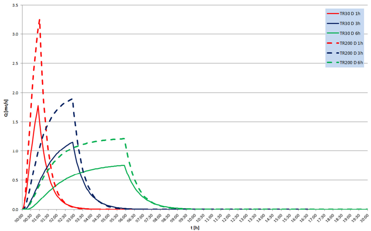
SEZ. 105 - 35 - UNIFORM LATERAL INFLOW HYDROGRAPH
