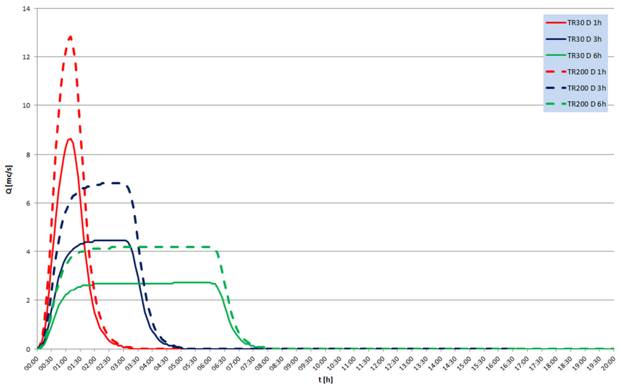
SEZ. 79.800 - 050 - UNIFORM LATERAL INFLOW HYDROGRAPH
