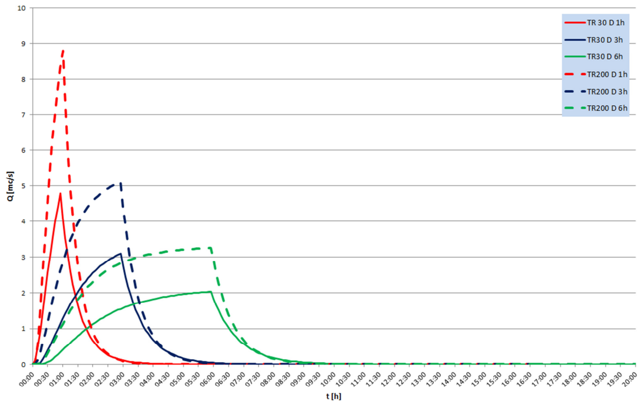
SEZ. 54 - 8 - UNIFORM LATERAL INFLOW HYDROGRAPH
