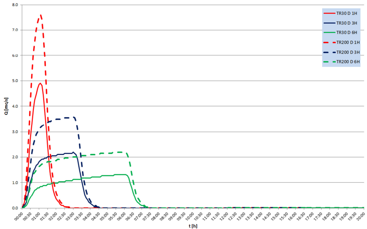
SEZ. 23 - FLOW HYDROGRAPH
