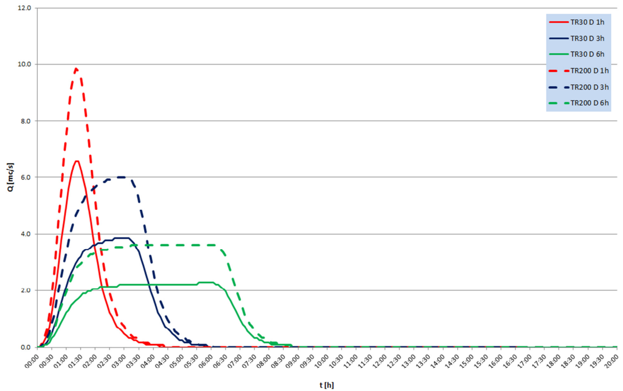
SEZ. 12 - FLOW HYDROGRAPH
