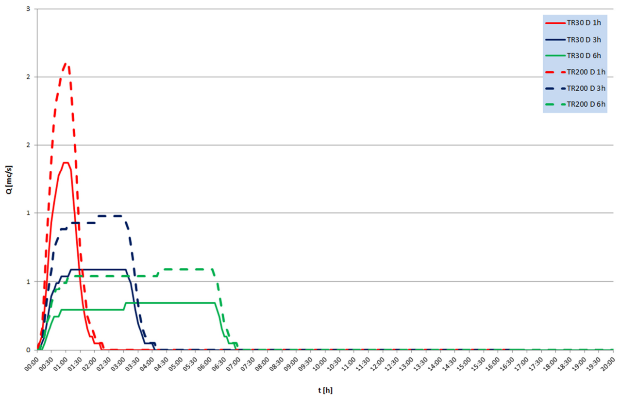
SEZ. 40.05 - 15 - UNIFORM LATERAL INFLOW HYDROGRAPH
