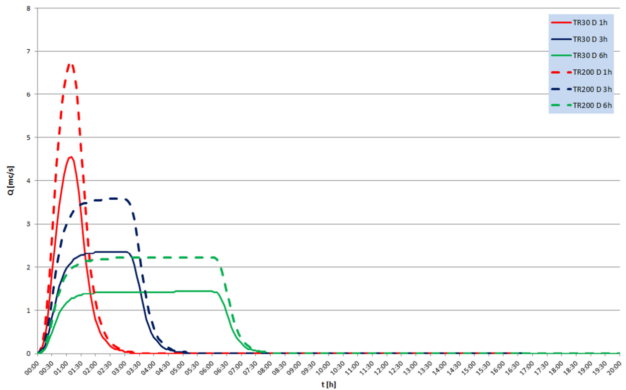
SEZ. 080 - FLOW HYDROGRAPH
