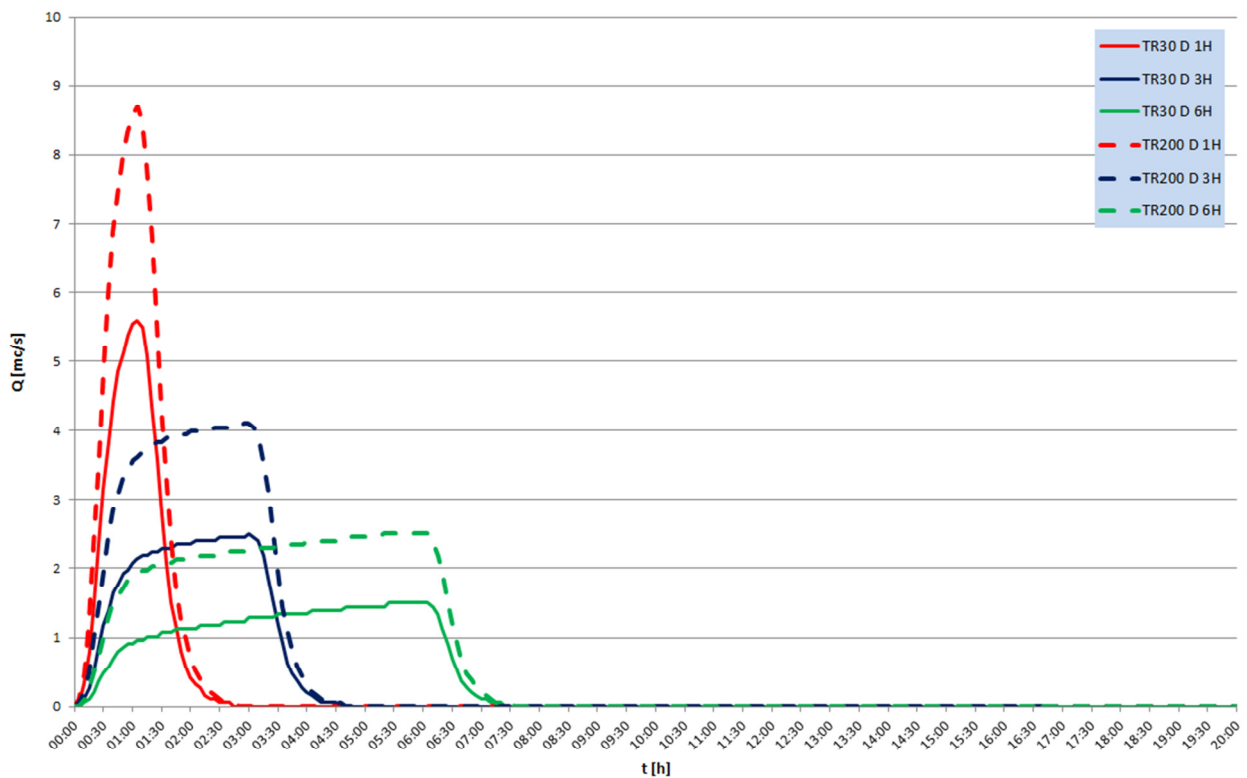
SEZ. 18-3 - UNIFORM LATERAL INFLOW HYDROGRAPH
