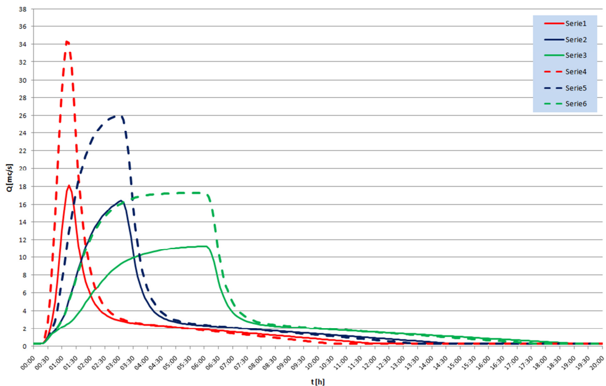
SEZ. 705 - LATERAL INFLOW HYDROGRAPH
