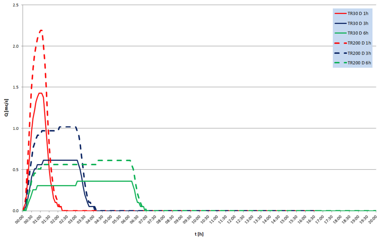
SEZ. 41.05 - FLOW HYDROGRAPH
