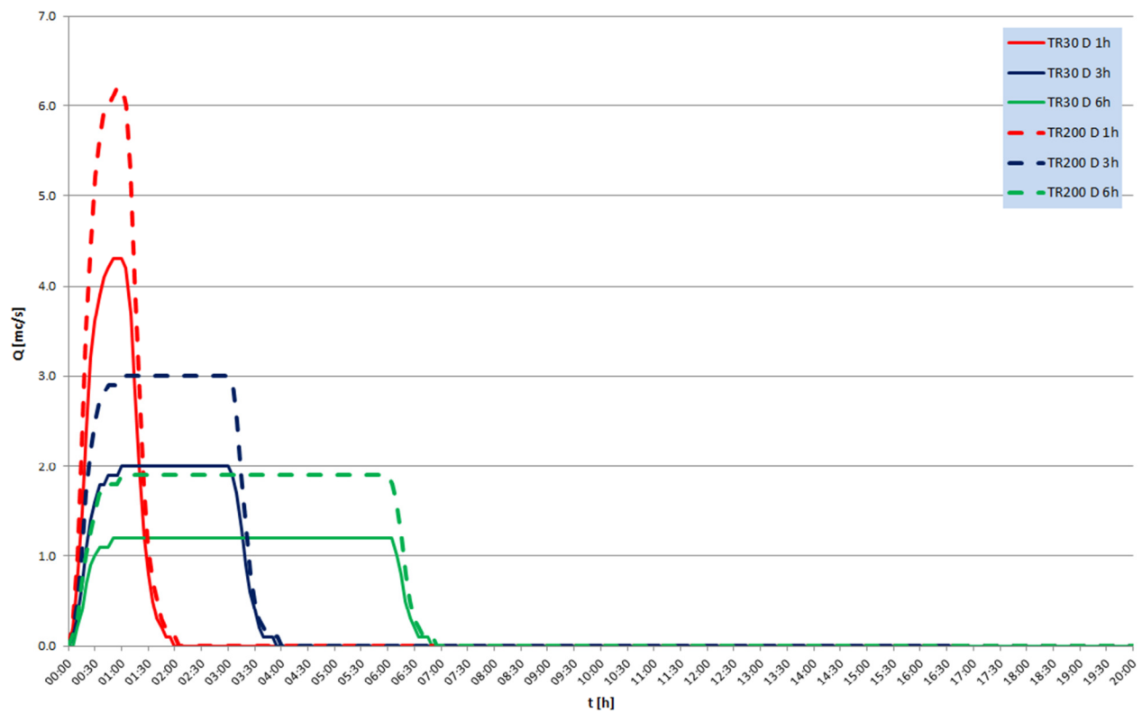
SEZ. 2264 - 1348.012 - UNIFORM LATERAL INFLOW HYDROGRAPH
