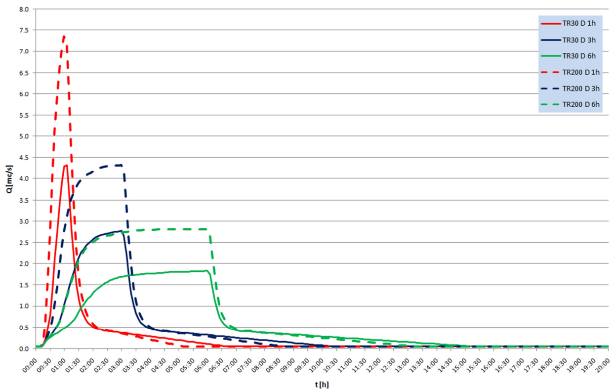
SEZ. 795 - LATERAL INFLOW HYDROGRAPH
