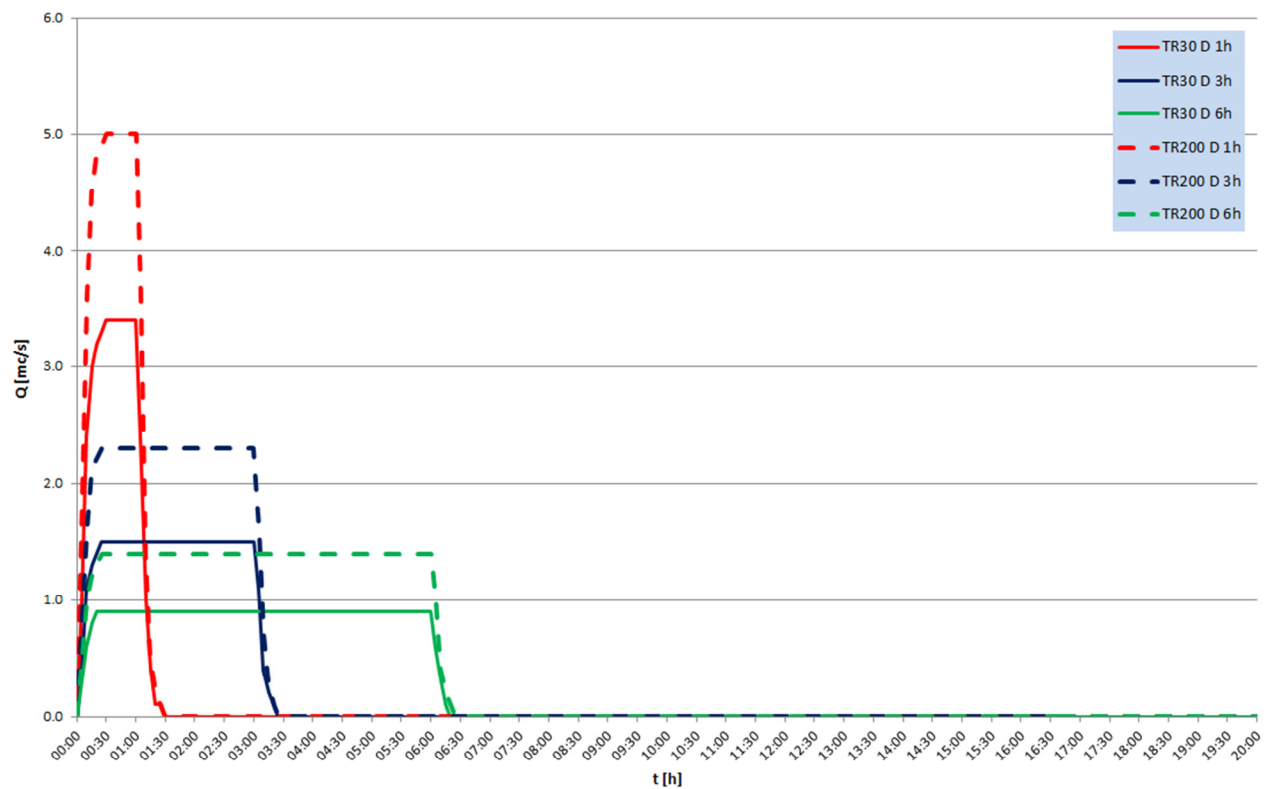
SEZ. 2566.1 - LATERAL INFLOW HYDROGRAPH
