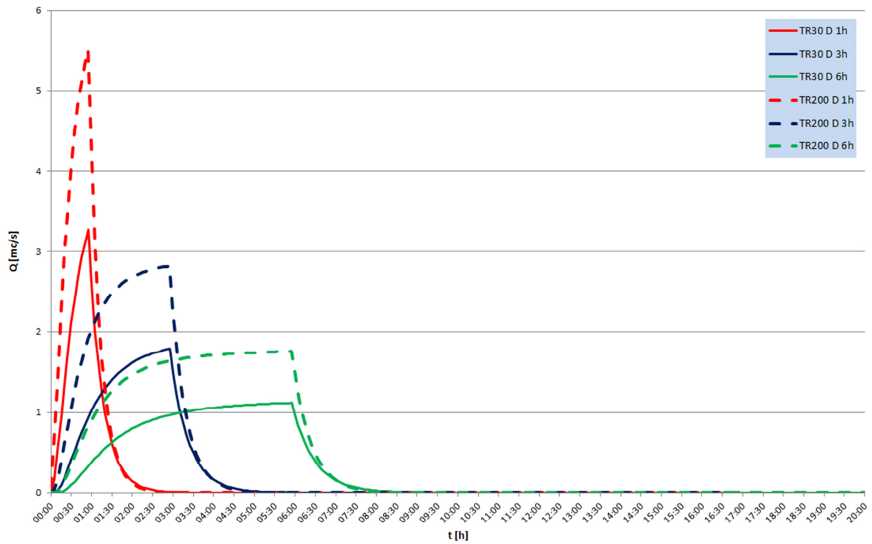
SEZ. 17 - FLOW HYDROGRAPH
