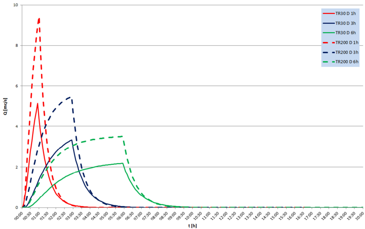
SEZ. 105 - 56 - UNIFORM LATERAL INFLOW HYDROGRAPH
