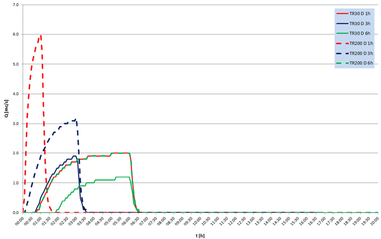
SEZ. 1000 - FLOW HYDROGRAPH
