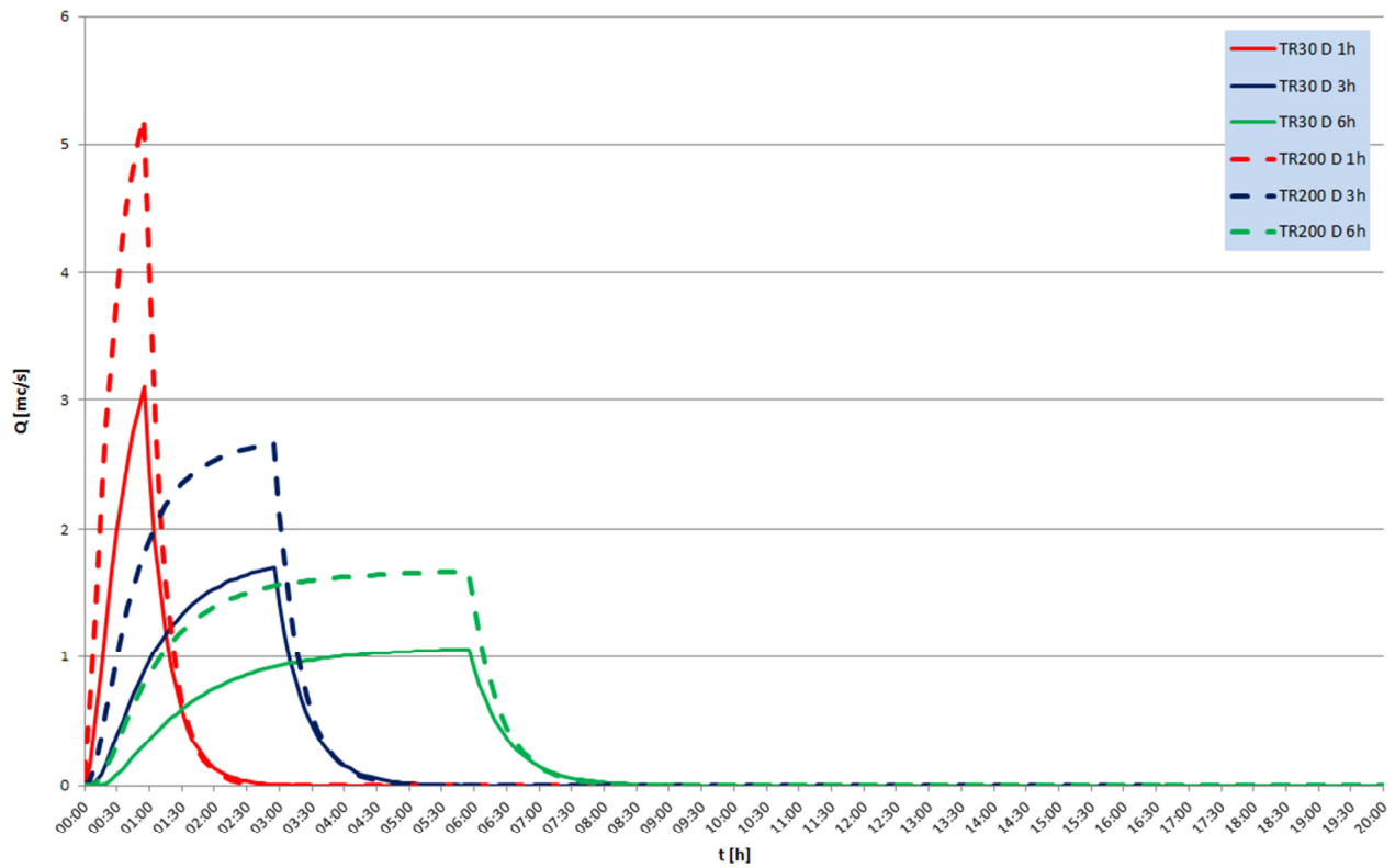
SEZ. 16 - LATERAL INFLOW HYDROGRAPH
