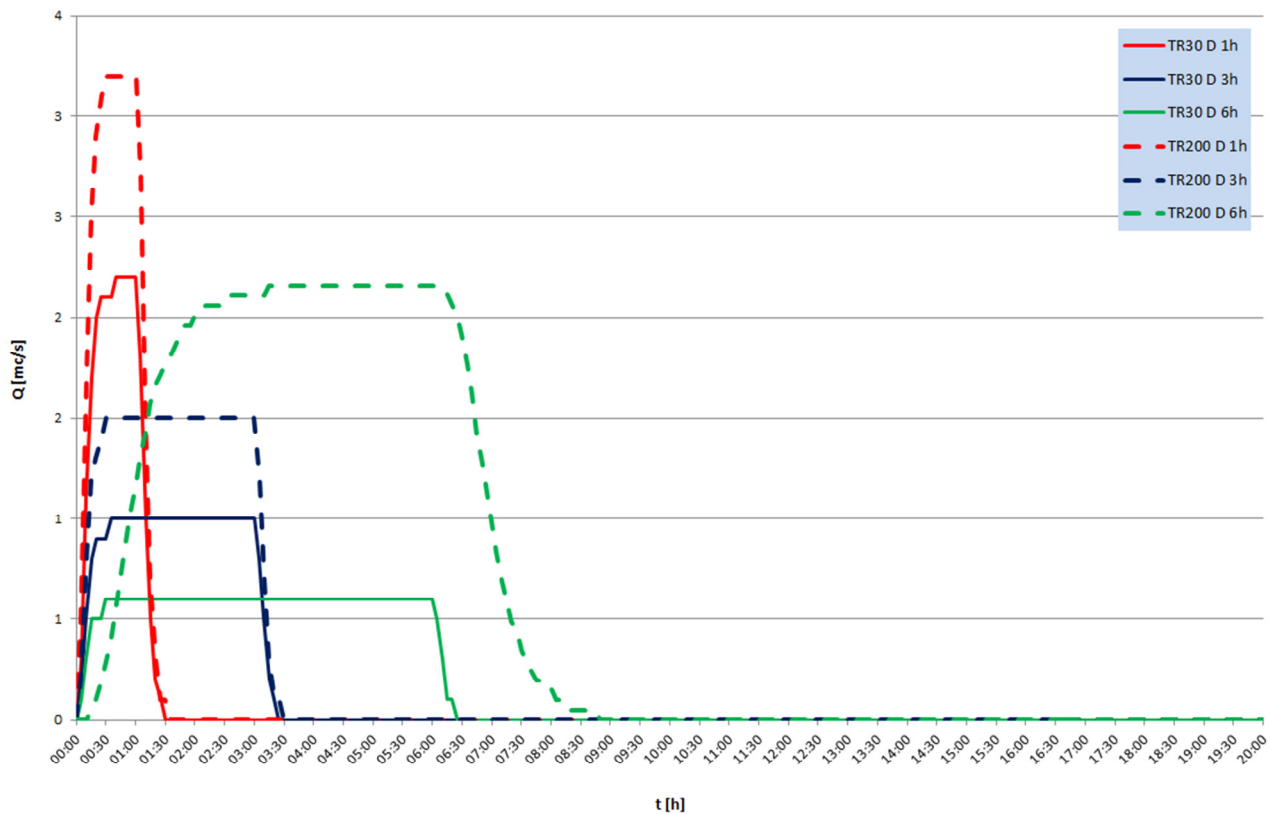
SEZ. 995 - LATERAL INFLOW HYDROGRAPH
