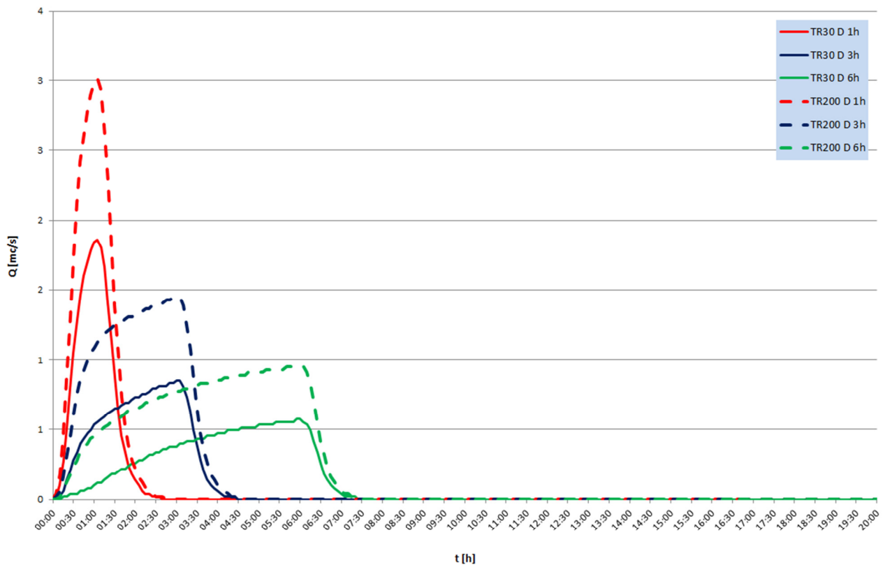
SEZ. 34 - 002 - UNIFORM LATERAL INFLOW HYDROGRAPH
