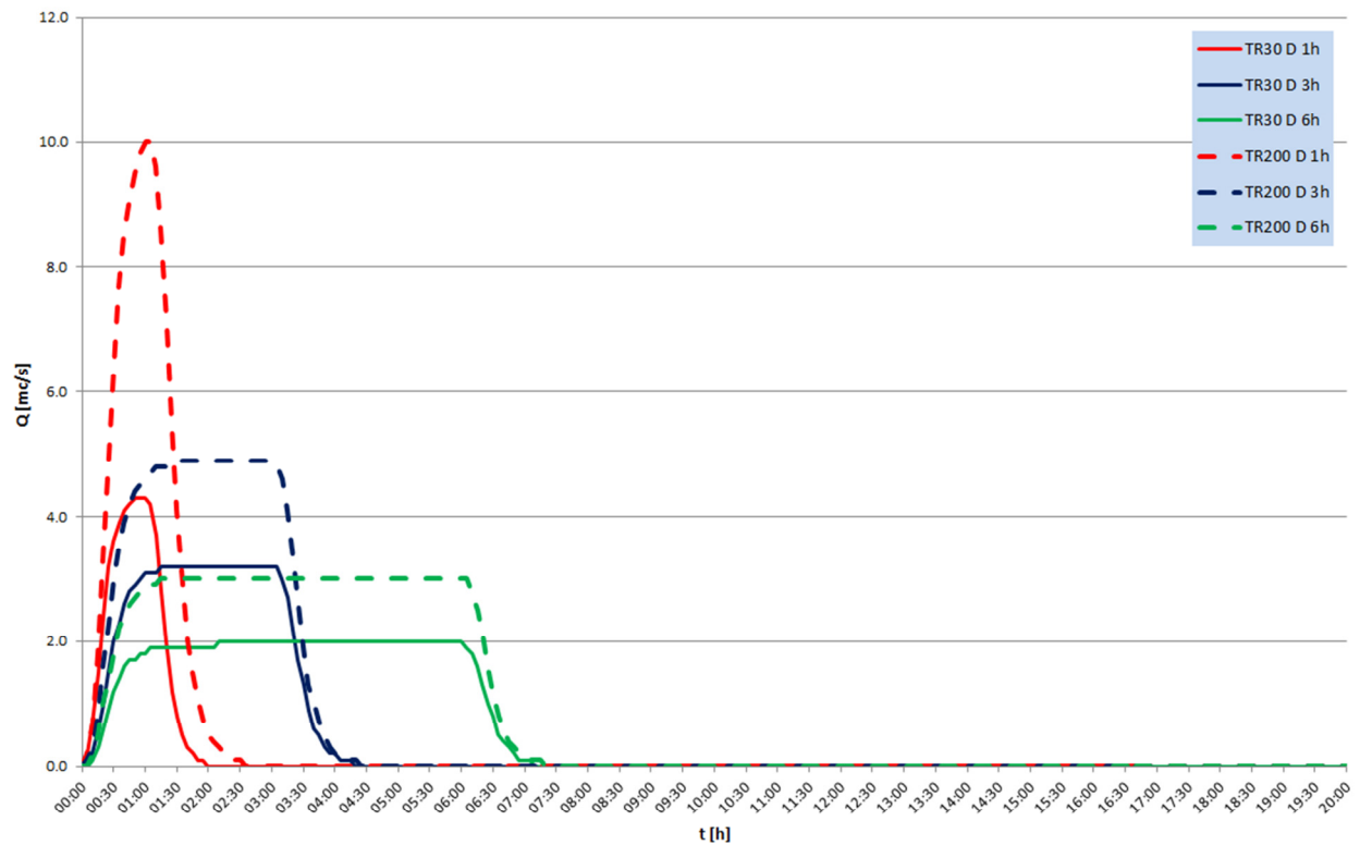
SEZ. 1710 - LATERAL INFLOW HYDROGRAPH
